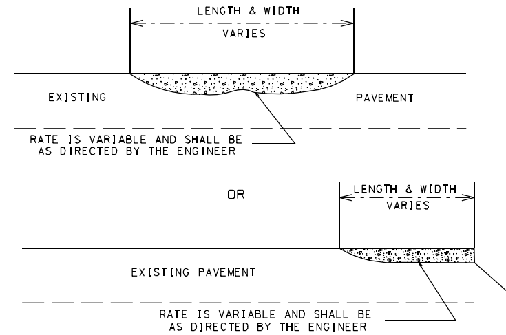
DETAIL B ASPHALT CONCRETE SURFACE COURSE TYPE S9.5B. (LEVELING COURSE) (AS NEEDED FOR LEVELING PATCHES)
