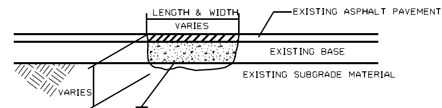
DETAIL A PATCHING EXISTING PAVEMENT
